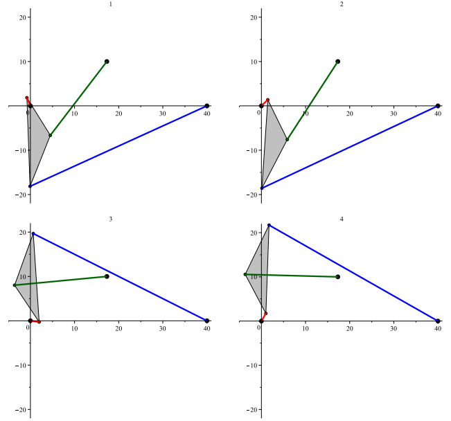
Fig. 8. The four moving platform poses obtained in Example V and their graphical representation.
