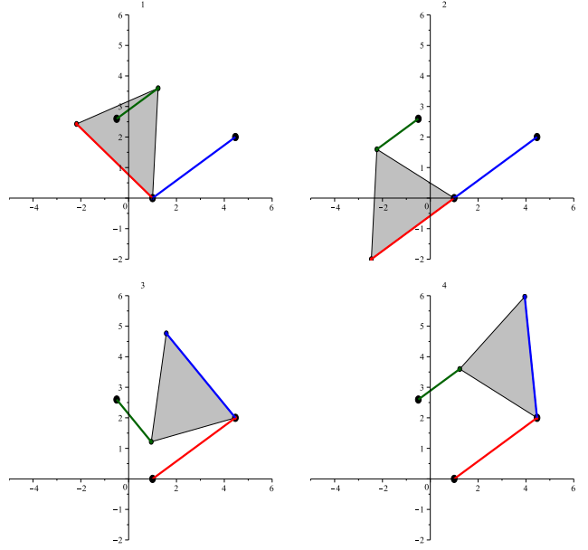
Fig. 5. The four moving platform poses obtained in Example II and their graphical representation.
