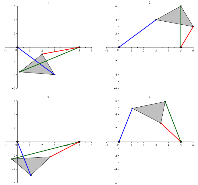
Fig. 6. The four moving platform poses obtained in Example III and their graphical representation.
