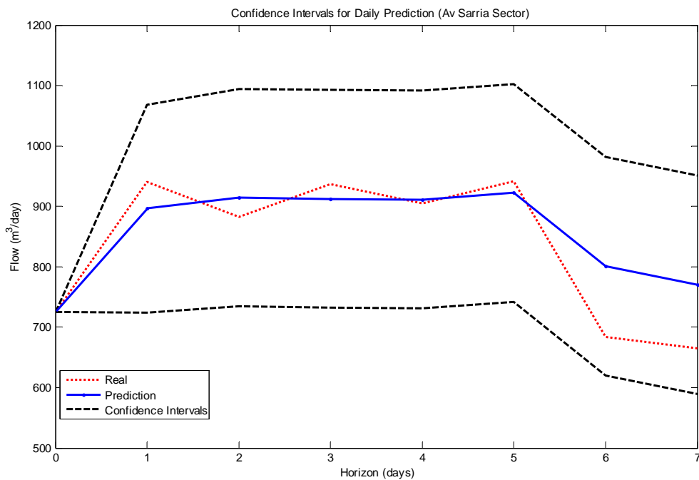
Fig. 8. Evolution of the daily flow prediction confidence intervals changing the horizon corresponding to “Avinguda Sarrià” sector
