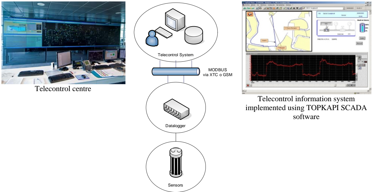
Fig. 2. Telecontrol of Barcelona water distribution system
