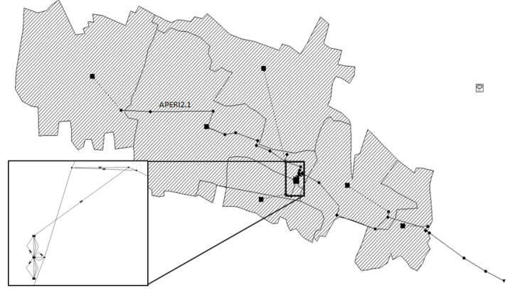
Fig. 5. SWMM configuration of the Perinot case study
