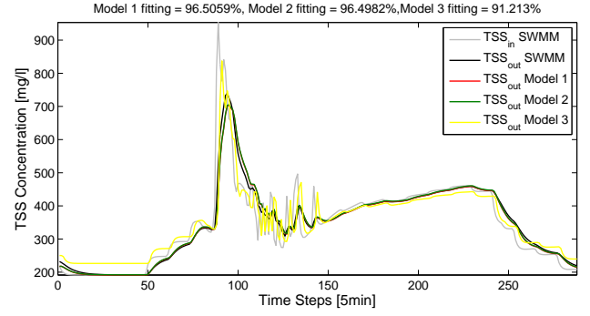
Fig. 9. V1 validation performance for T1
