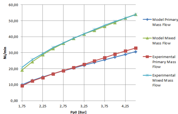
Figure 4. NXP=3.5 mm, P_{p0}=1.2 \text{ bar}_{\text{abs}}
