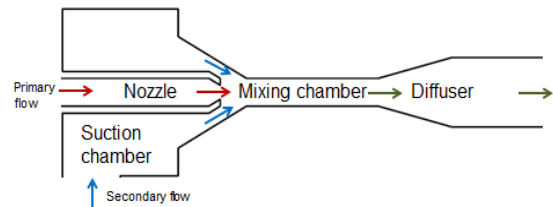
Figure 2. Ejector schematic.
