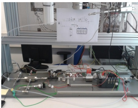
Figure 3. Experimental set-up
