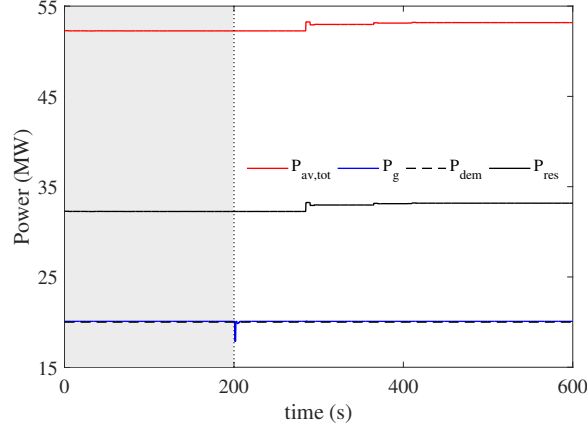
Figure 6: Scenario 1: Power evolution for v_\infty = 11 m/s with a direction of 0 degrees.
