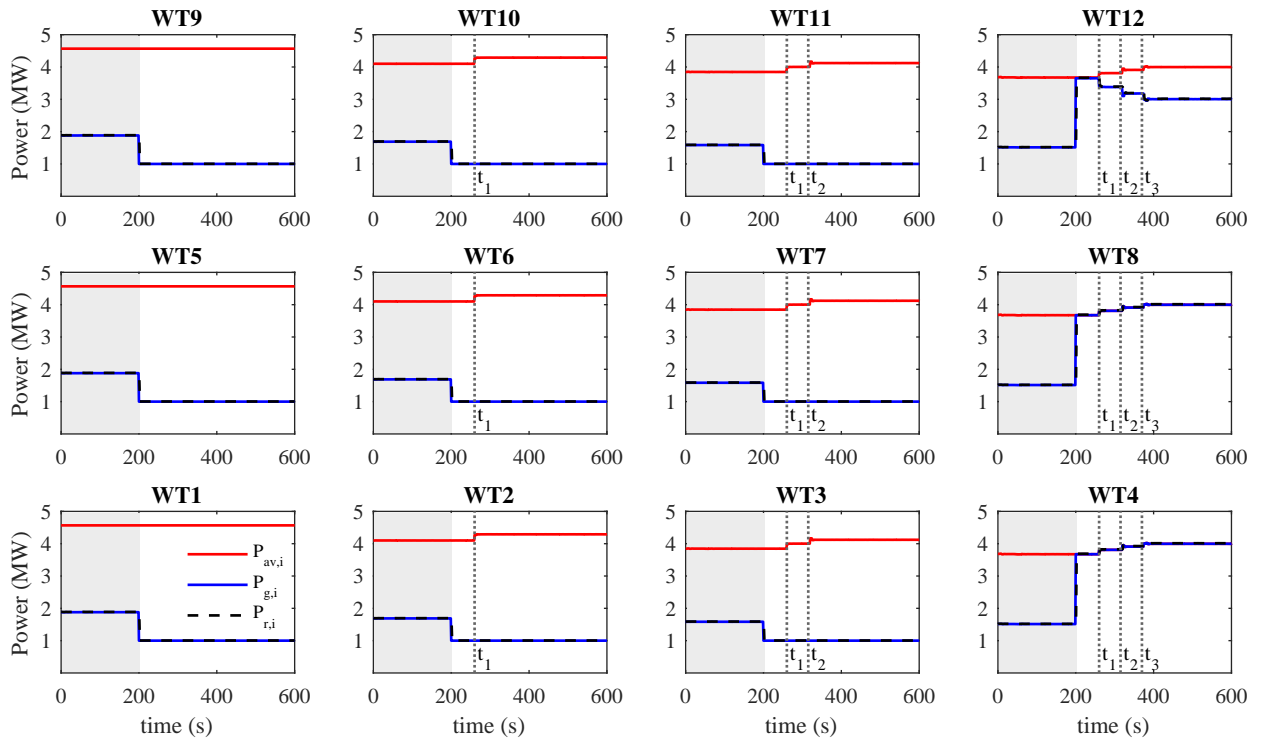
Figure 7: Scenario 1: generated ( P_{g,i} ), available ( P_{av,i} ) and set-point ( P_{r,i} ) powers for each wind turbine. Shadow area: baseline power distribution function. White area: proposed distribution algorithm.
