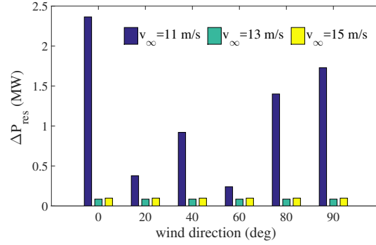
Figure 10: Scenario 2: Summary of power reserve levels obtained with the proposed algorithm for several free-stream wind speeds and directions.
