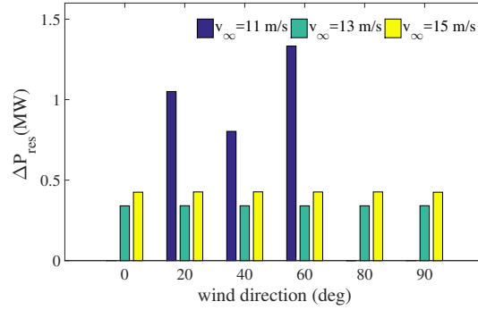
Figure 12: Scenario 3: Summary of power reserve levels obtained with the proposed algorithm for several free-stream wind speeds and directions.
