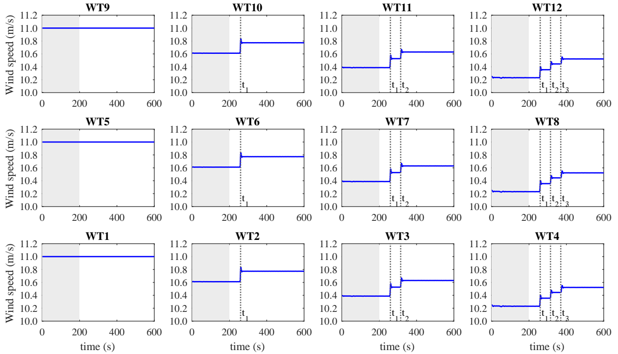
Figure 8: Scenario 1: wind speeds faced by each turbine. Shadow area: baseline power distribution function. White area: proposed distribution algorithm.
