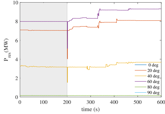
Figure 11: Scenario 3: power reserve for several wind directions, P_{\text{dem}} = 45 MW, v_{\infty} = 11 m/s.
