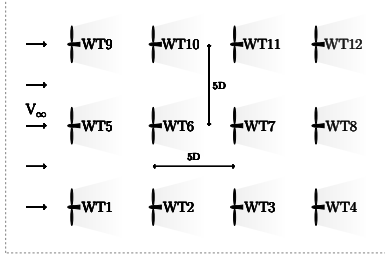
Figure 4: Wind farm layout corresponding to the case study. The turbines are considered oriented to the free-stream wind speed direction.
