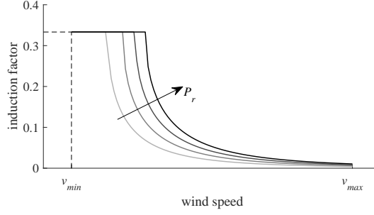
Figure 2: Induction factor a – wind speed v characteristic for several power set-points P_r . The black line corresponds to the nominal case ( P_r = P_{\text{rated}} ).
