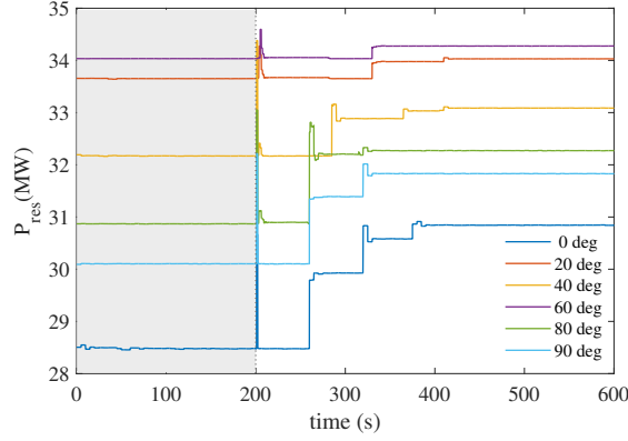
Figure 9: Scenario 2: power reserve for several wind directions, P_{\text{dem}} = 20 MW, v_{\infty} = 11 m/s.
