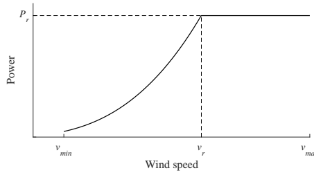
Figure 3: Available power – wind speed v characteristic.
