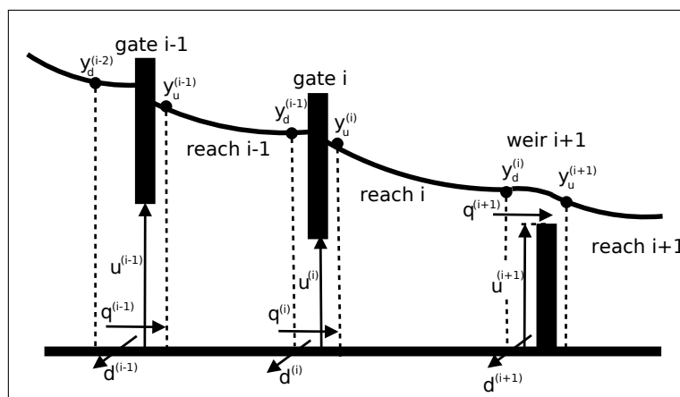
Figure 3: Navigation canal schematic with the variables involved
