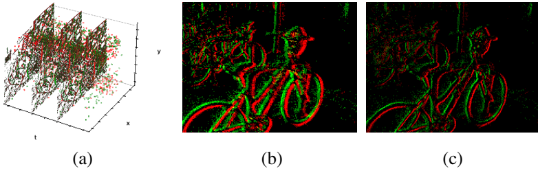
Figure 1: Input data and optimization: (a) event input data with polarity in red and green and aggregated counts in black, (b) event count image with event counts represented by intensity, (c) deblurred image of warped events (IWE) after motion compensation.
