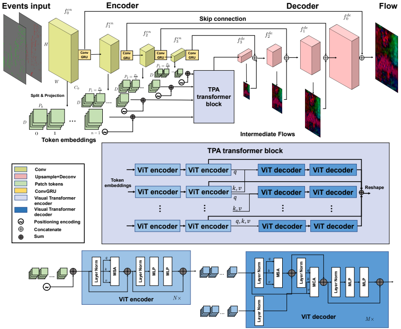
Figure 2: ET-FlowNet architecture.
