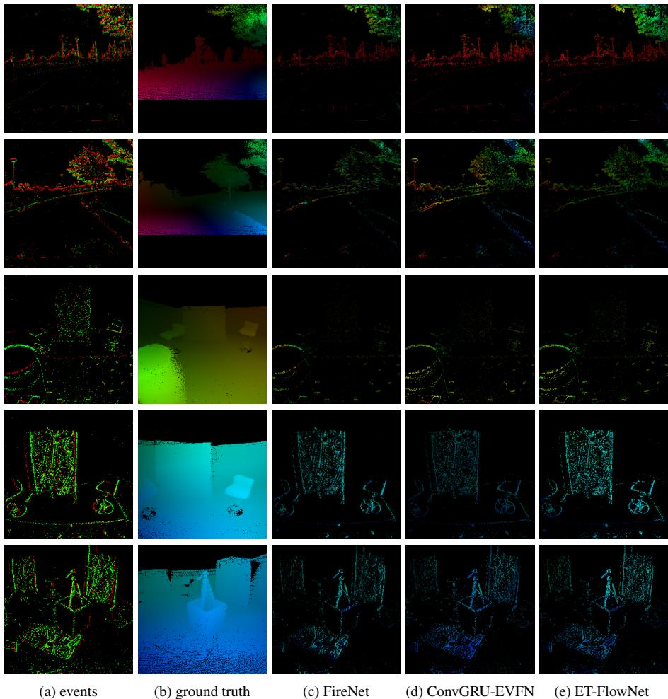
Figure 3: Qualitative results for optical flow evaluated on the MVSEC dataset for the dt = 1 case. Top two rows are from outdoor_day1 sequence and the last three are from indoor_flying1, indoor_flying2 and indoor_flying3 sequences, respectively. The first column presents the event input and the second column shows the ground truth dense optical flow provided in the MVSEC dataset (Note that for evaluation we use the masked sparse optical flow). Compared to other self-supervised methods trained also on different datasets: (c) FireNet and (d) ConvGRU-EV-FlowNet, our method (e) ET-FlowNet shows qualitatively better results on the outdoor sequences and competitive results in the indoor sequences (best viewed in color).
