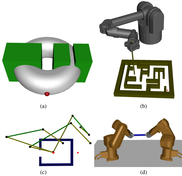
Fig. 5 The four benchmarks used to test the AtlasRRT planner. (a) A small sphere moving on a torus with obstacles and a narrow corridor. (b) The Barret arm solving a maze problem. (c) A planar parallel manipulator moving a peg out of a cul-de-sac. (d) Two Stäubli Rx60 industrial arms collaborating to move a cylindrical bar.
