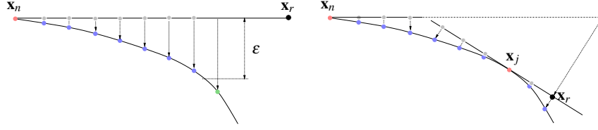
Fig. 4 RRT extension on a one-dimensional cut. The RRT is extended towards \mathbf{x}_r , the randomly selected point, from \mathbf{x}_n , the closest point already in the tree. In this case, \mathbf{x}_n is the center of a chart. When the extension reaches a point (the green dot) where the error with respect to the chart at \mathbf{x}_n is larger than \epsilon , a new chart is created from the previous node already in the tree and \mathbf{x}_r is projected to the new chart. Then, the RRT extension continues in the new chart until the projected \mathbf{x}_r is reached.
