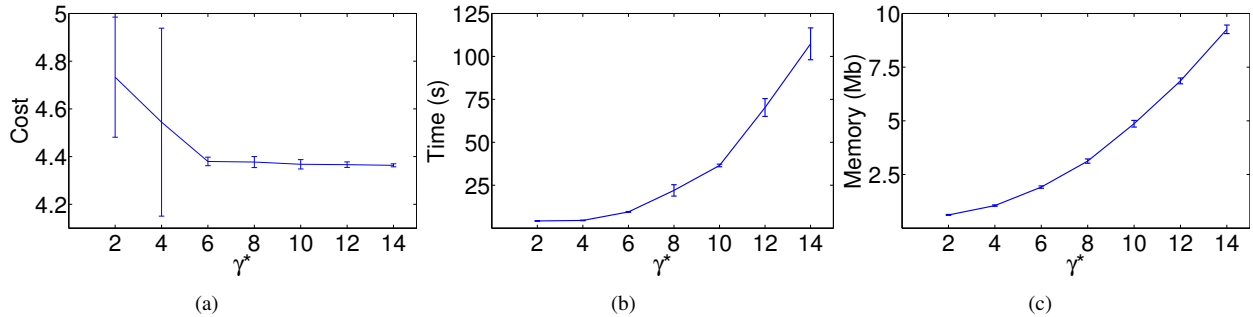
Figure 7: Path cost, execution time (in seconds), and memory use in megabytes (Mb) for the AtlasBiRRT* planner on the torus example for different values of \gamma^* after 10000 iterations.
