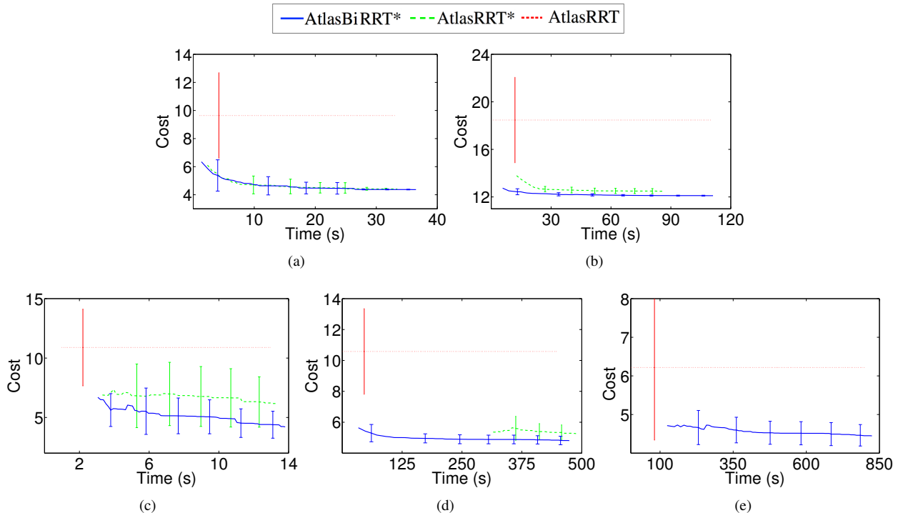
Figure 5: Path cost versus execution time for the AtlasBiRRT*, AtlasRRT*, and AtlasRRT planners on (a) the torus, (b) the cyclooctane, (c) the Barrett, (d) the PR2, and (e) the Robot Hand problems averaged over 25 executions. Costs are given once a solution is found in at least 70% of the repetitions. In the Robot Hand problem the AtlasRRT* planner finds the solution in only one of the 25 repetitions and, thus, it is not shown in the corresponding plot. In the plots, the vertical bars give the standard deviation.
