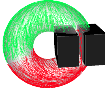
Figure 2: A bidirectional RRT* constructed on a torus-like manifold. The two RRT trees are shown in red and green, respectively.
