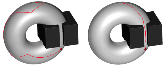
Figure 1: Two paths connecting the same query configurations for a small ball moving on a torus while avoiding obstacles. Left A jerky path obtained with a standard sampling-based path planner. Right A close-to-optimal solution when optimizing the path length.
