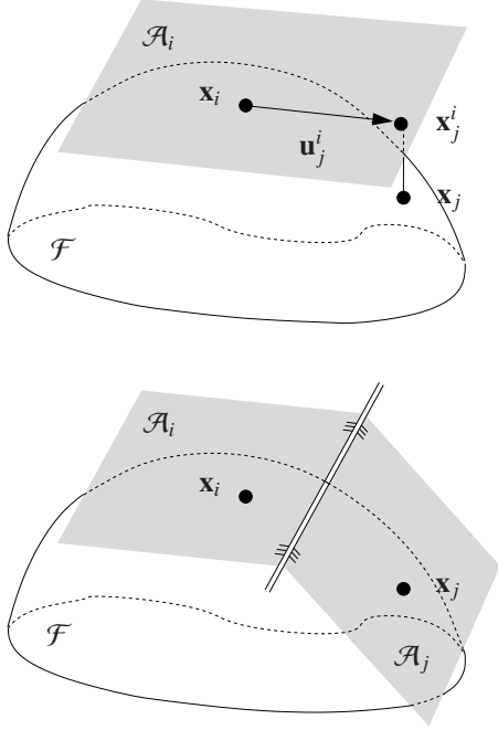
Figure 3: Top A generic approximation of the exponential map is obtained by orthogonally projecting to \mathcal{F} a point \mathbf{x}_j^i on the tangent space at \mathbf{x}_i . Bottom When a new chart is defined at \mathbf{x}_j , the applicability areas of the two charts, \mathcal{A}_i and \mathcal{A}_j , are coordinated to avoid overlaps and to keep track of the part of the manifold already parametrized.
