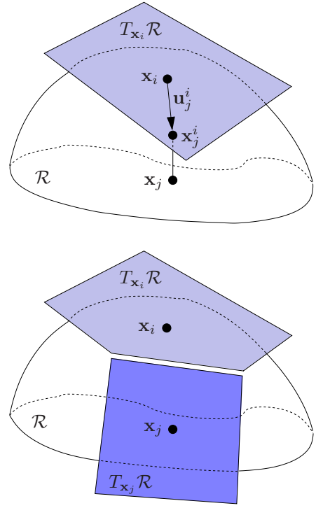
Fig. 4. The higher-dimensional continuation method applied to a two-dimensional manifold \mathcal{R} in 3D space. Using the chart centered at \mathbf{x}_i , a point \mathbf{x}_j^i on the chart corresponding to a vector \mathbf{u}_j^i \in T_{\mathbf{x}_i}\mathcal{R} is orthogonally projected to obtain a point \mathbf{x}_j \in \mathcal{R} (top). If a new chart is defined at \mathbf{x}_j , it must be properly coordinated with the chart at \mathbf{x}_i so that their projections smoothly cover the manifold (bottom).
