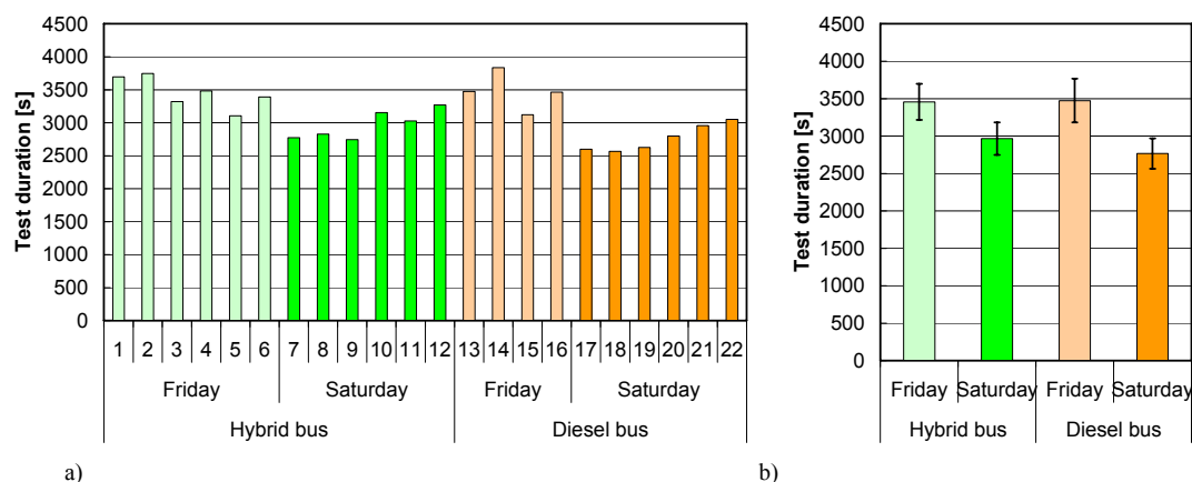
Figure 2. The comparison of the test duration for the hybrid and conventional buses: a) all runs, b) average values with the measurement uncertainty marked
