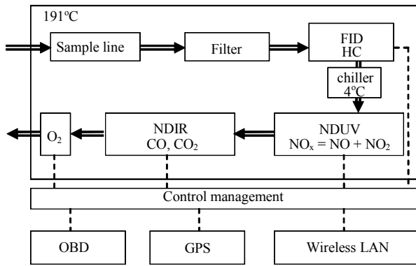
Figure 4. A diagram of a mobile analyzer SEMTECH DS; exhaust gas flow channels (==) and electrical connections circled (---)
