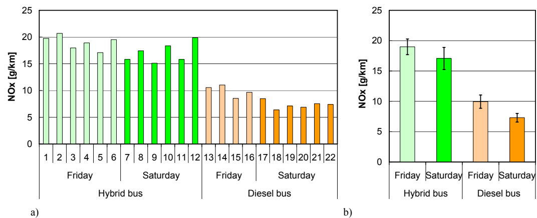
Figure 8. The comparison of the road emission of nitrogen oxides during the testing of the hybrid and conventional buses: a) all runs, b) average values with the measurement uncertainty marked
