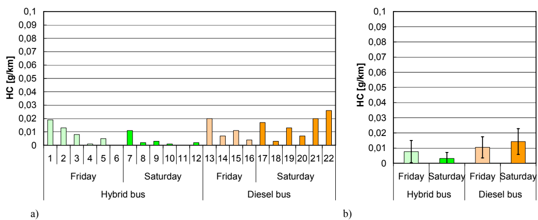
Figure 7. The comparison of the road emission of hydrocarbons during the testing of the hybrid and conventional buses: a) all runs, b) average values with the measurement uncertainty marked
