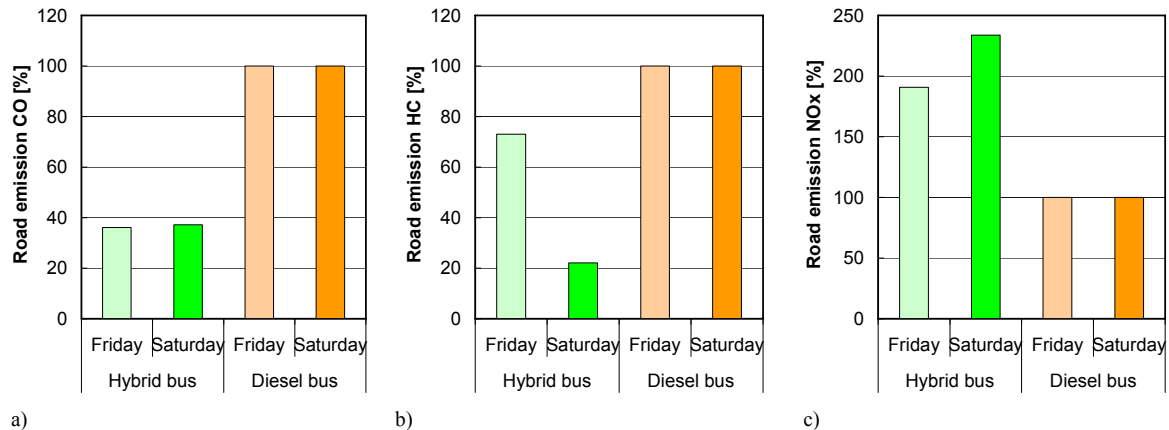
Figure 9. Relative change in the road emissions of the hybrid as opposed to the conventional one (for which the reference values of 100% were adopted): a) carbon monoxide, b) hydrocarbons, c) nitrogen oxide
