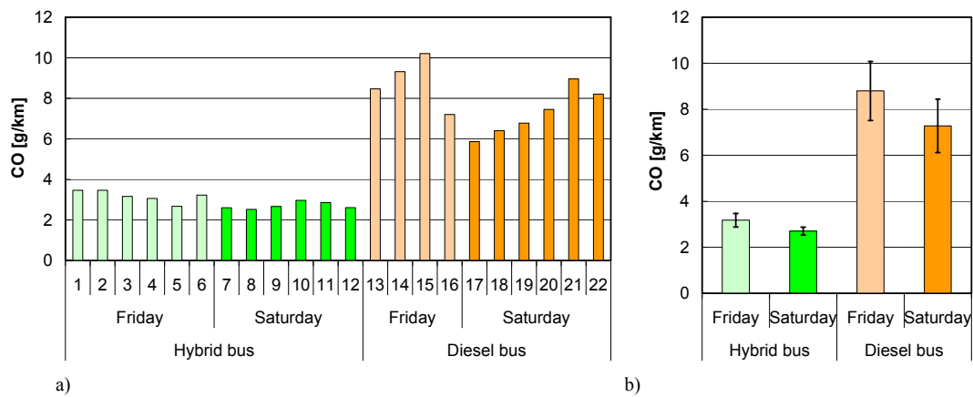
Figure 6. The comparison of the road emissions of carbon monoxide during the testing of the hybrid and conventional buses: a) all runs, b) average values with the measurement uncertainty marked
