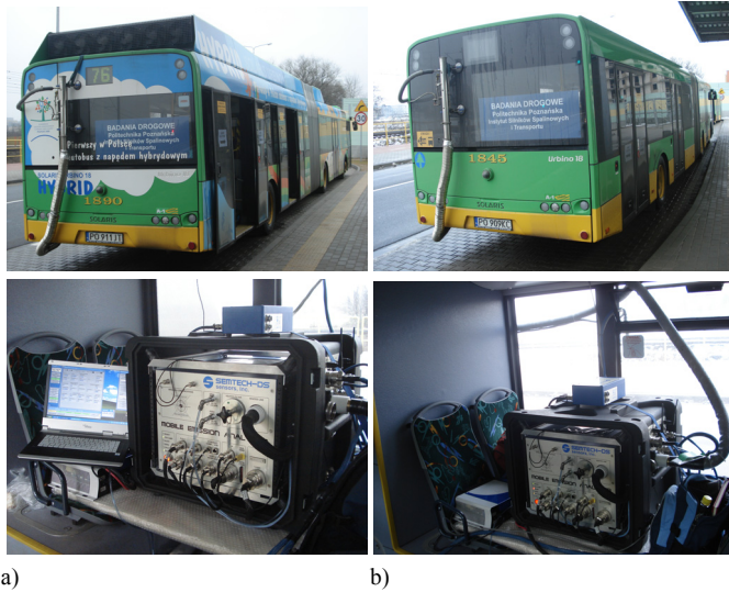
Figure 5. The view of the measuring equipment (exhaust emission measurement unit Semtech DS) fitted in the bus during the tests: a) hybrid, b) conventional
