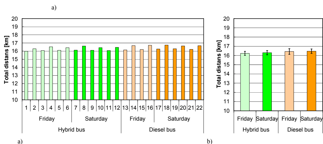
Figure 3. The comparison of the total test distance for the hybrid and conventional buses: a) all runs, b) average values with the measurement uncertainty marked
