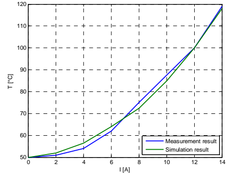
Figure 9. Comparison of temperature from simulation and measurement
