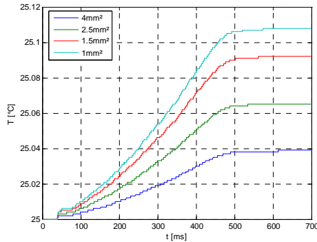
Figure 16. Parameter variation of conductor size of wire 7
