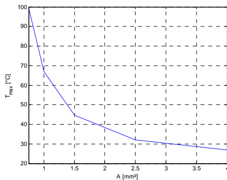
Figure 17. Maximum conductor temperature for a current loading of 130 A
