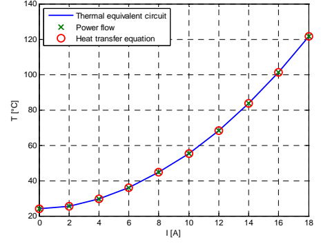
Figure 2. Comparison of different approaches for steady state
