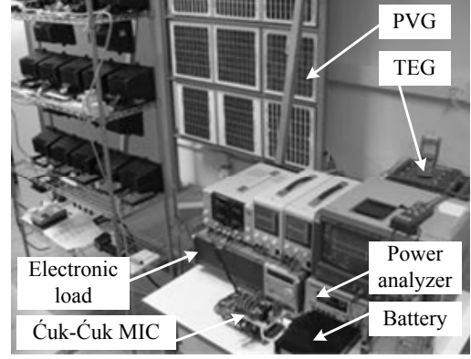
Fig. 4. System prototype.
