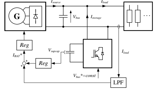
Figure 4. “Dual” control strategy
