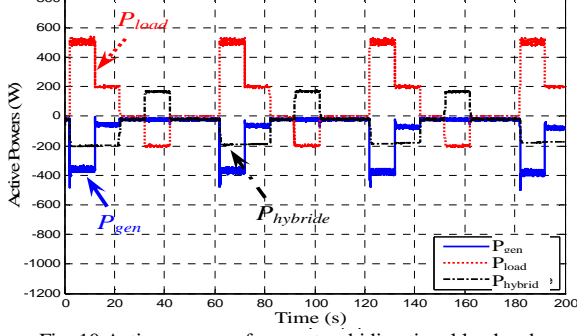
Fig. 10 Active powers of generator, bidirectional load and hybrid system with PI+FC strategy
