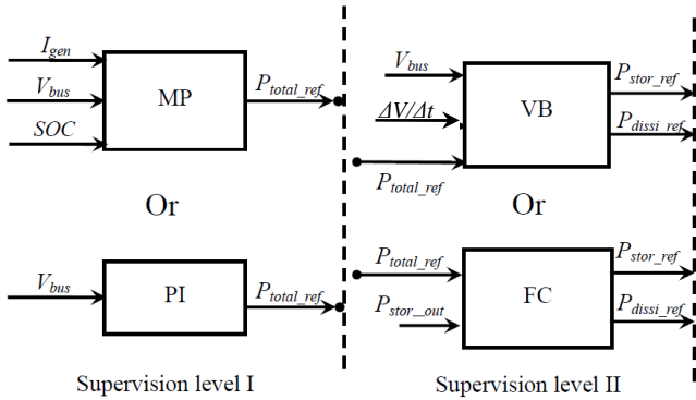
Fig. 4 Global structure of each power management strategy
