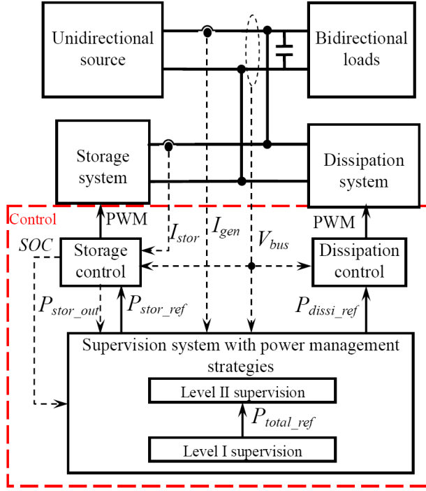
Fig. 3 Supervision architecture.
