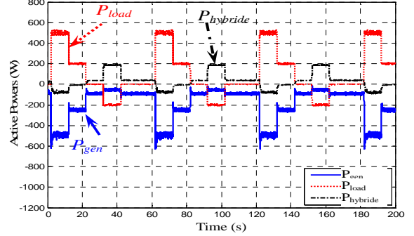
Fig. 14 Active powers of generator, bidirectional load and hybrid system with MP+VB strategy
