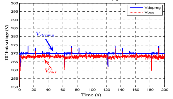
Fig. 13 DC-link voltage evolution with MP+VB strategy
