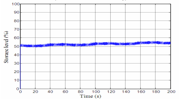
Fig. 16 Supercapacitor energy storage level for MP+VB strategy
