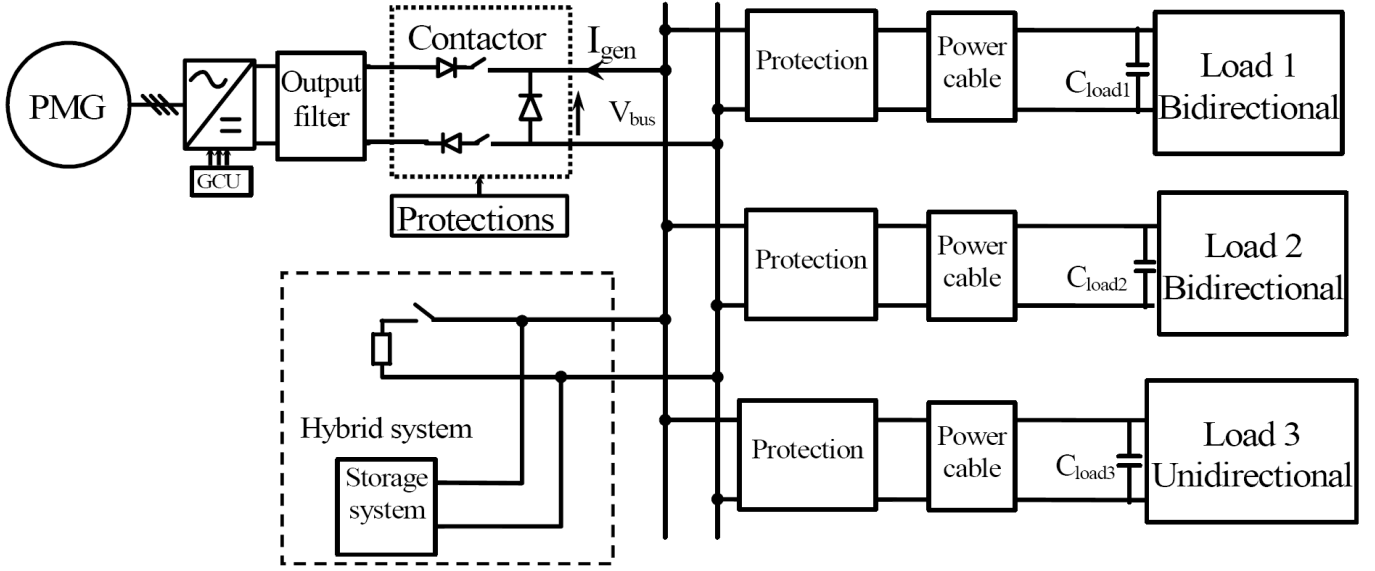
Fig. 1 Local DC on-board network with hybrid storage and dissipation system.
