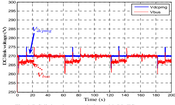
Fig. 9 DC-link voltage evolution with PI+FC strategy
