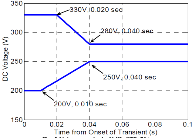
Fig. 2 Voltage standard of MIL-STD-704.
