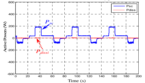
Fig. 15 Active powers for the hybrid storage and dissipation system with MP+VB strategy
