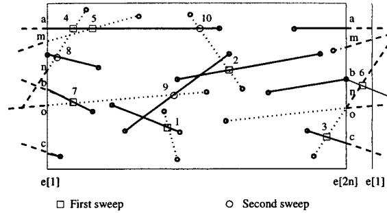
Figure 3: Plane analogue of the spherical sweep. Red and blue arcs are depicted as dotted and solid segments. Some of them ( a, b, c, m, n, o ) begin before or at the last event point n_i and end after the first one n_1 . These segments are activated during the first sweep from e[1] to e[2n] , where some purple intersections can already be detected (marked with a small square), and their intersections with the segments that had ended before they were generated (marked with an empty circle) can only be detected during a second sweep. Numbers indicate the order in which the intersections are computed.
