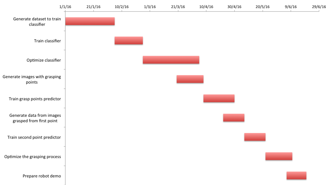
Figure 1.3: Gantt Diagram.
