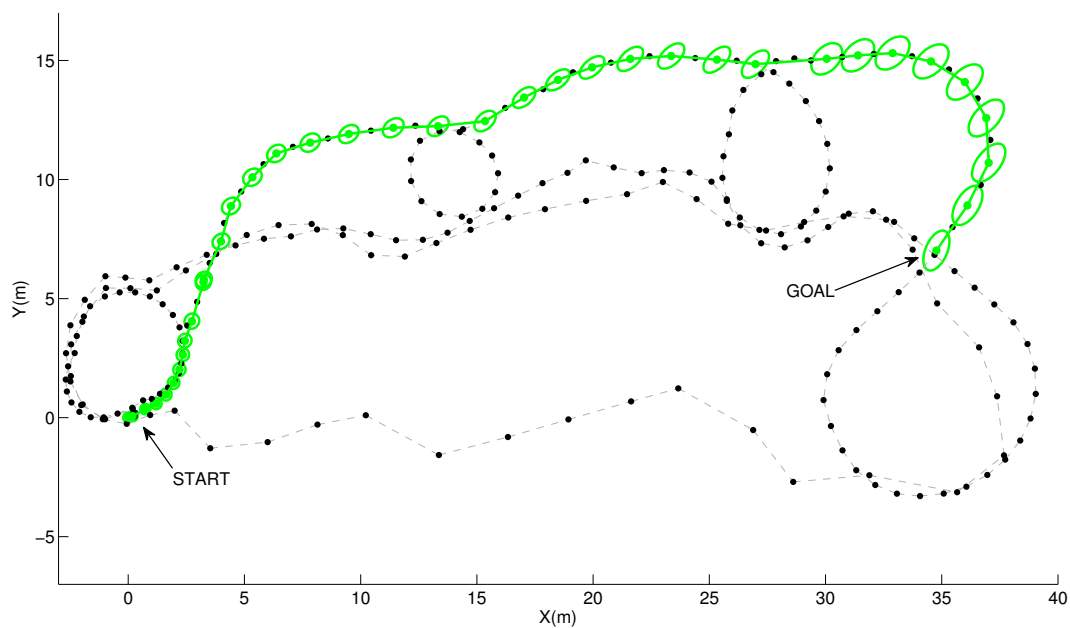
(b) Minimum uncertainty path to the goal.
