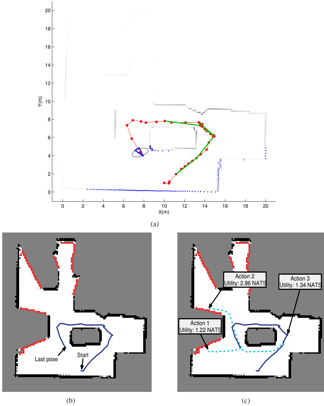
Figure 5.1: The Pose SLAM posterior is used to render an occupancy map, which is used to generate candidate paths. (a) Pose SLAM map. (b) Gridmap and frontiers (red cells). (c) Candidate paths and their utilities.
