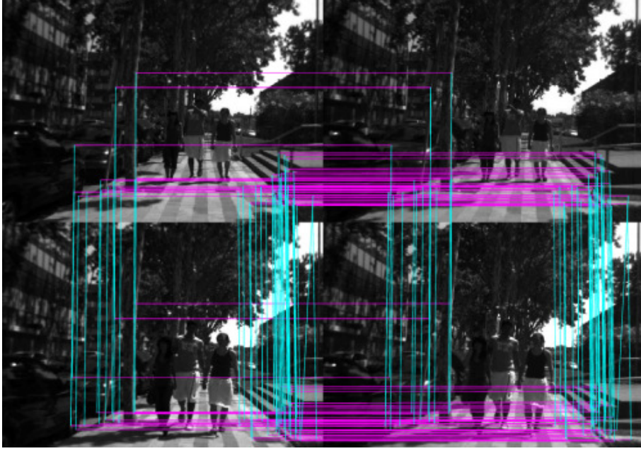
Figure 2.1: SIFT correspondences in two consecutive stereo image pairs after outlier removal using RANSAC.
