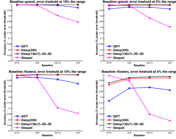
Fig. 6. Baseline results.
