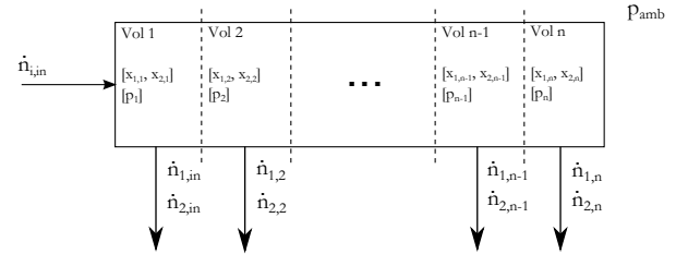
Fig. 2. Generalized model of the discretized anode gas channel
