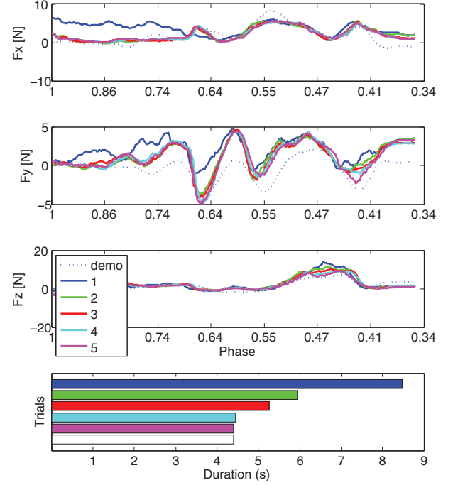
Fig. 18. The upper three graphs show the sensed forces during trajectory execution (solid lines) and the forces recorded during training (dashed lines), all as a function of phase. The bar graph below shows the execution time in each learning cycle.
