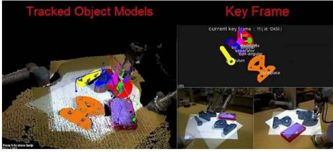
Fig. 7. The IntelliAct vision system: On the left, the tracking history at an intermediate stage of the assembly is shown. The coloured threads show the positions each moved object has gone through during the assembly process. The picture on the top right shows the poses found. The two pictures on the bottom right show two images of the cameras.
