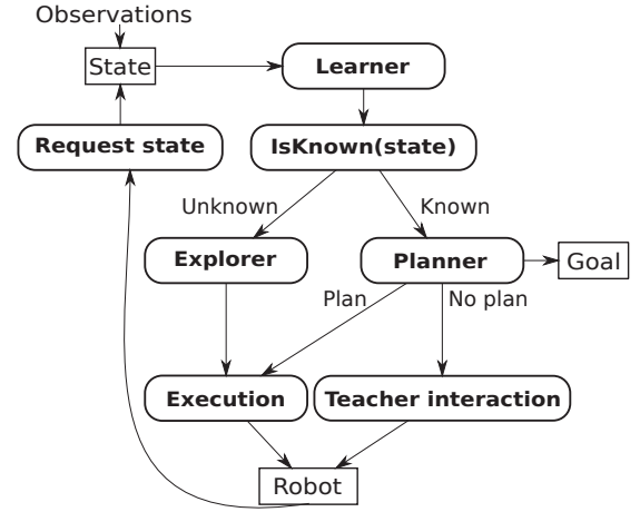
Fig. 16. Overview of the REX-D algorithm.
