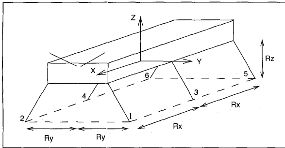
Figure 1: Reference posture for the six-legged robot Genghis II.
