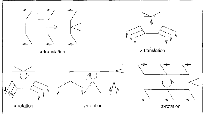
Figure 4: The five approximate conservative gestures for a six-legged robot with 2-DOF legs.
