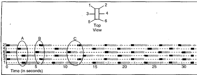
Figure 5: Gait obtained on a smooth surface.
