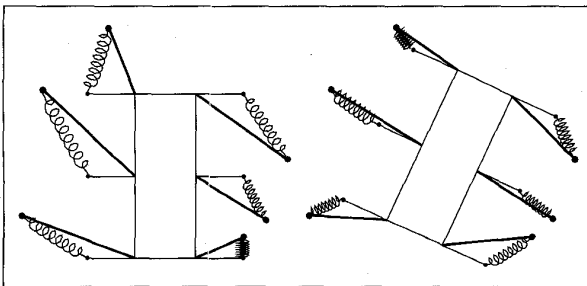
Figure 2: Physical interpretation of the optimal posture (in two dimensions). At left, a six-legged robot in an arbitrary posture is shown. Actual robot legs are represented in thick lines. Big dots correspond to actual feet positions, which must remain fixed. In thin lines, the body of the robot is represented with imaginary rigid legs positioned in the reference posture. Springs connecting the vertices of the actual and reference feet positions exert a force and torque on the body of the robot. The right figure shows the position to which the springs would drive the body, and corresponds to the optimal posture.
