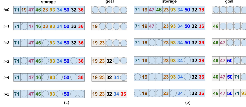
Fig. 3. Example of two traces or play-outs, provided by a caregiver to teach the “ascending order” exercise. Both traces are meant to demonstrate the same exercise. In (a) the caregiver teaches how to sort the five smallest numbers while in (b) he teaches how to sort the five largest numbers. In both traces, the initial token position ( t = 0 ) is random. Later steps ( t > 0 ) show the progress of the caregiver in the current trace.
