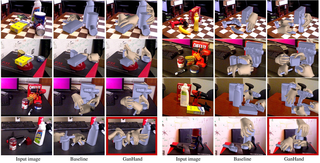
Figure 7: Sample results on the YCB-Affordance. Failure cases in bottom row: The absolute pose of the can and clamps is not accurate and overlapping grasps are produced (left). The cup is detected as a brick, predicting a wrong grasp (right).
