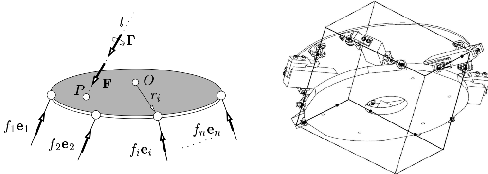
Figure 1: Left: A platform connected to its environment through n legs. Right: Conceptual design of the sensor. Legs of length 0.1 m are aligned with the edges of a cube of side 0.3 m.
