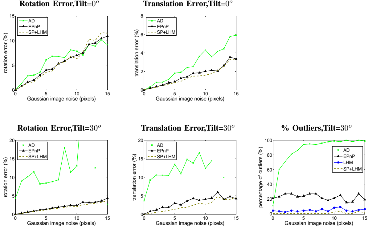
Fig. 7. Planar case. Errors as a function of the image noise when using n = 6 reference points. For Tilt=0°, there are no pose ambiguities and the results represent the mean over all the experiments. For Tilt=30°, the errors are only averaged among the solutions not affected by the pose ambiguity. The right-most figure represents the number of solutions considered as outliers, which are defined as those for which the average error in the estimated 3D position of the reference points is larger than a threshold.
