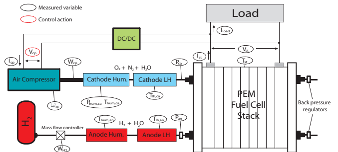
Figure 2: PEM Fuel cell system schematics
