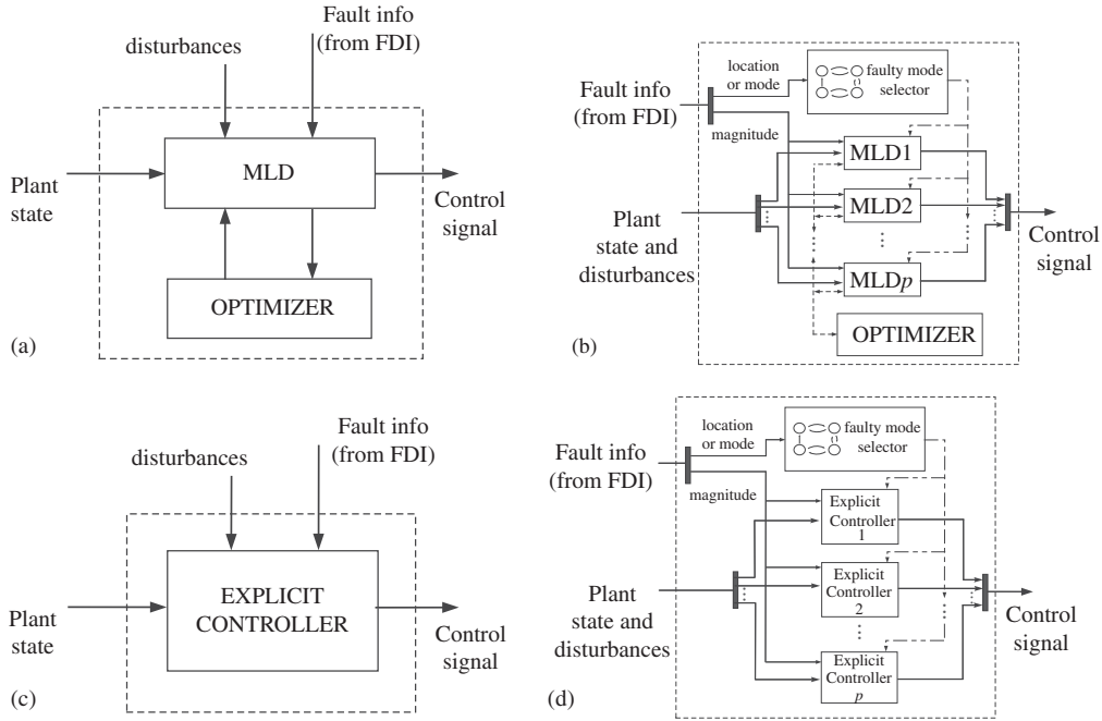
Figure 7. Implementation architectures for FTHMPC: (a) controller A; (b) controller B; (c) controller C; and (d) controller D.
