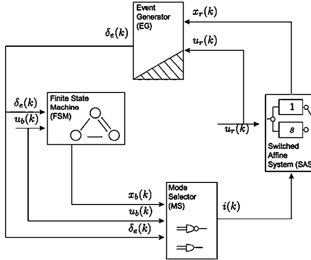
Figure 1. Discrete hybrid automata (taken from [12]).
