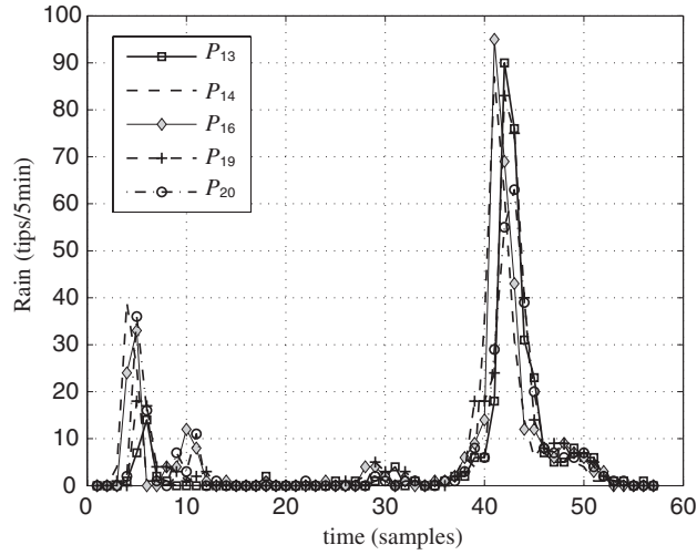
Figure 11. Rain episode occurred on 17 October, 1999 in Barcelona. Each curve represents a rain gauge P_i .
