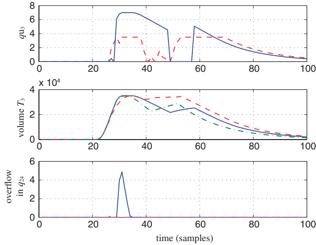
Figure 13. Network behavior for fault scenario f\bar{q}_{u_3} . PFTHMPC (—), AFTHMPC(---) and non-faulty HMPC (-.-) (rain episode: 03-09-1999).
