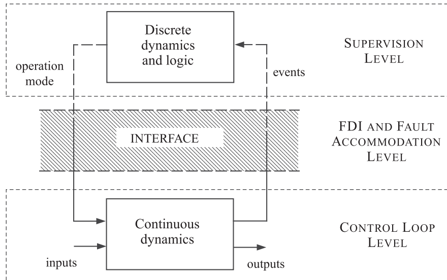
Figure 2. Parallelism between the basic scheme of a hybrid system and the three levels of an FTC architecture.
