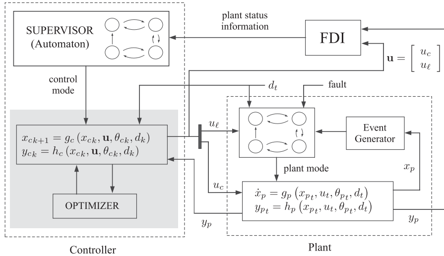
Figure 4. Scheme of the AFTHMPC architecture.
