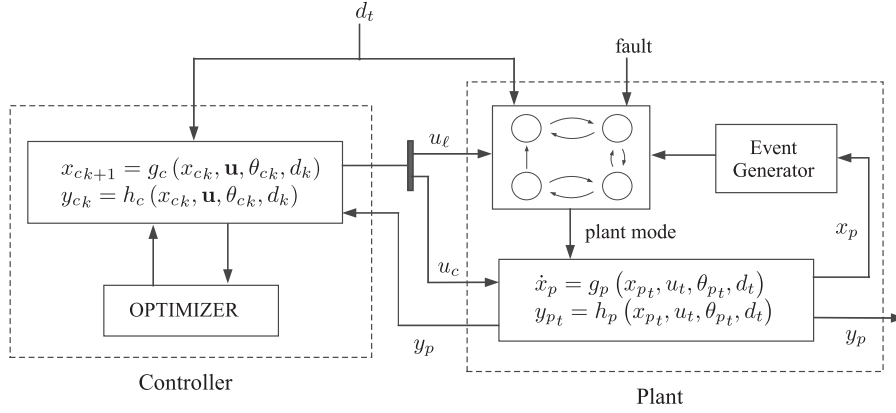
Figure 5. Scheme of the PFTHMPC architecture.
