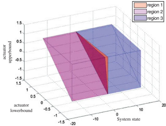
Figure 6. Polyhedra partitions of control law (14).
