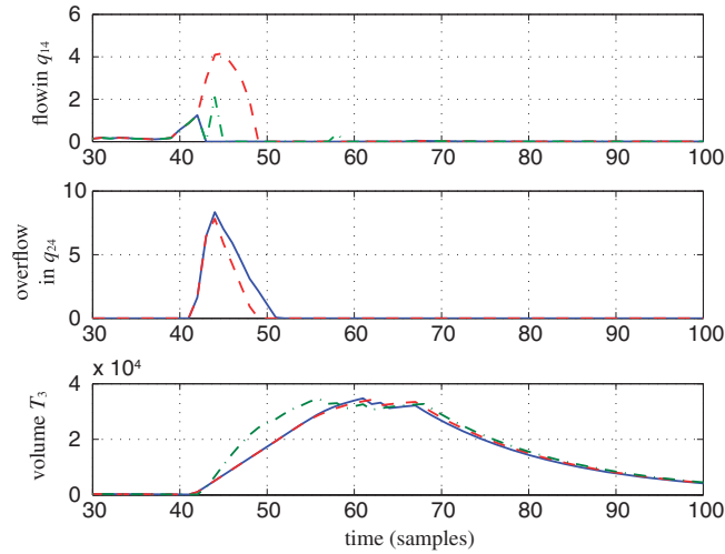
Figure 12. Set of actions in different parts of the test catchment for both active and passive FTHMPC approaches for fault scenario f\bar{q}_{u_2} . Solid curve (—): PFTHMPC; dashed curve (---): AFTHMPC; dotted-dashed curve (-.-): no-fault HMPC (rain episode: 17-10-1999).
