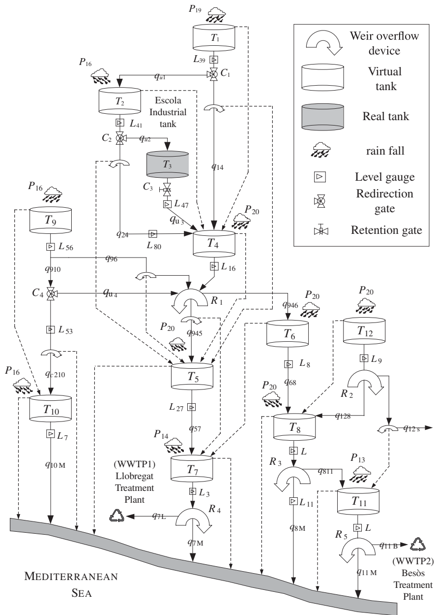
Figure 9. Barcelona test catchment scheme for hybrid design.
