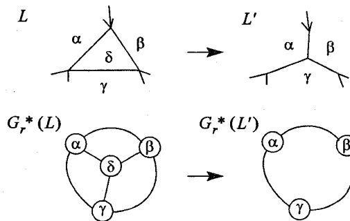
Fig. 6. Proof of the theorem for n=k+1 : \Delta \rightarrow Y case.
