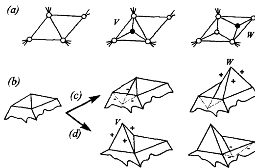
Fig. 8. Convexity and concavity emerges
