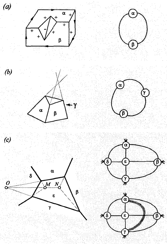
Fig. 1. Edge-alignment (a), edge-concurrence (b) and n -calotte (c) conditions.
