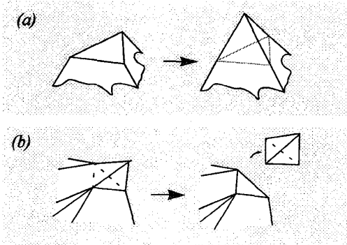
Fig. 2. Simplicial completion (a) and elimination (b).
