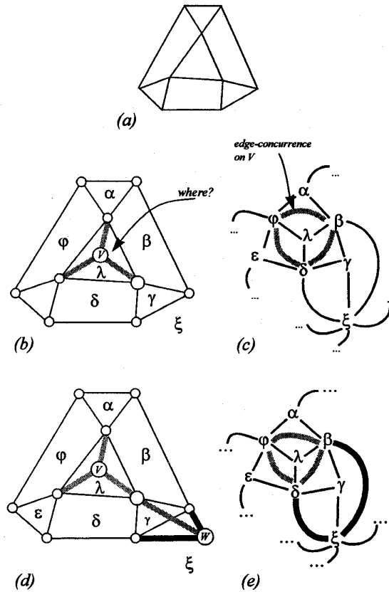
Fig. 5. Checking the consistency of a truncated pyramid.
